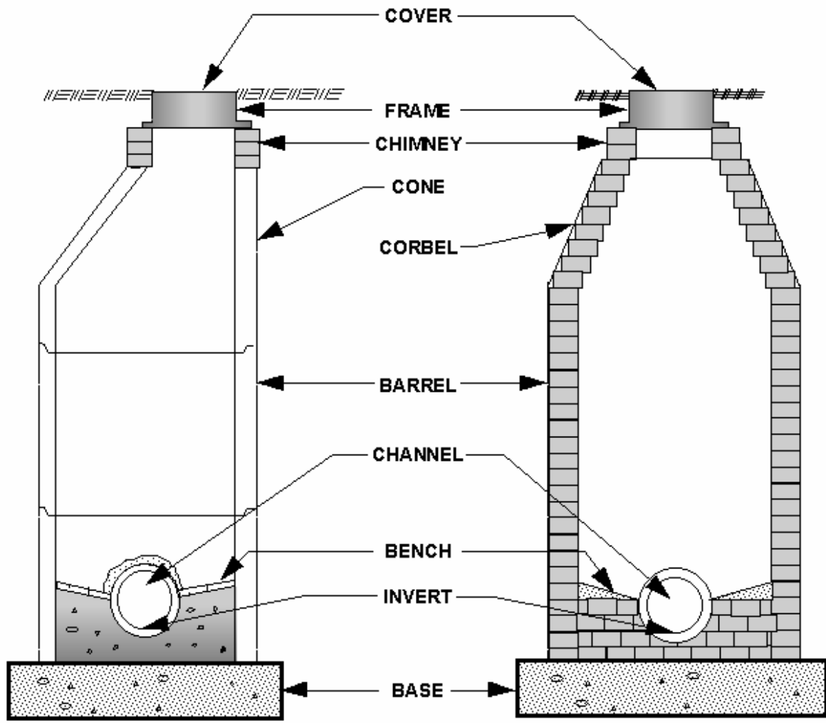
TYPICAL PRE-CAST MANHOLE
